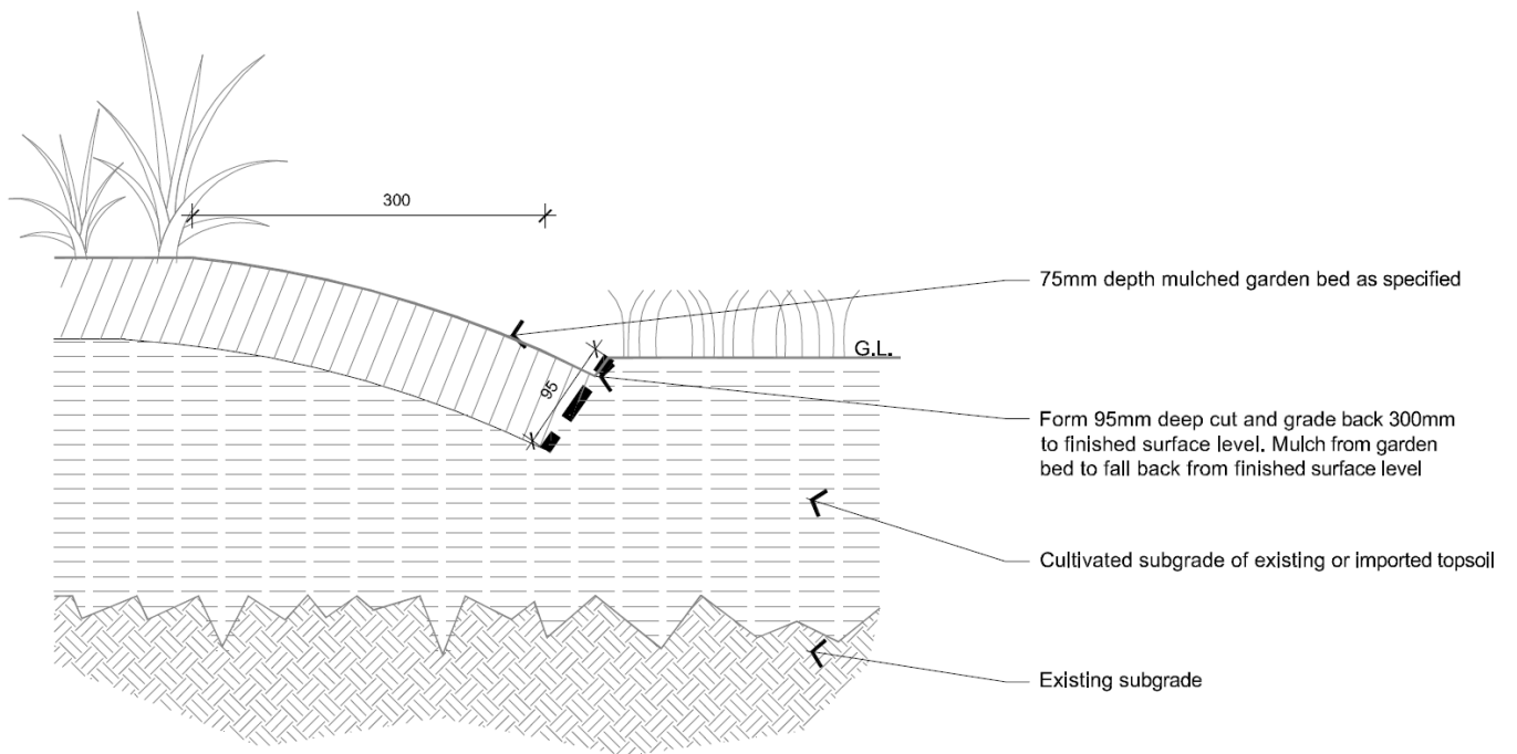
01 SPADE EDGING Detail 1:5
